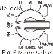
Fig 6 Mode Selector
